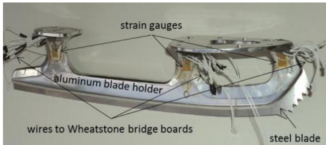
Hybrid skate with strain gauges and wires leading from gauges to Wheatstone bridge boards. Credit: IOP Publishing
