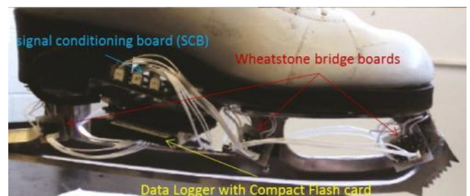
Instrumented ice skating blade integrated into boot system. Credit: IOP Publishing
