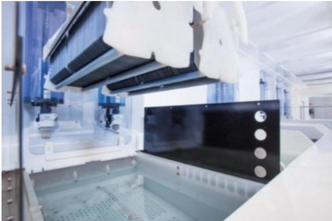
RENA BatchTex N process tank
