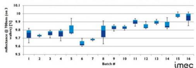
Reflectance of cz-wafers processed with monoTEX F based texturing chemistry, measured at 700 nm. As guidance 9.9 % @ 700 nm = 11.31 AWR
