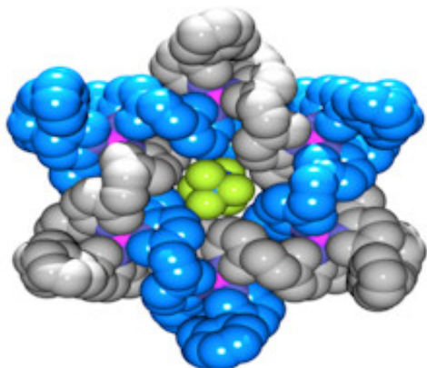
Atoms in the Star of David molecule. Credit: University of Manchester
