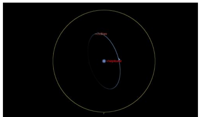
The orbit of Triton on the evening of August 29th, superimposed on a one arc minute field of view. Created using Starry Night Software.
