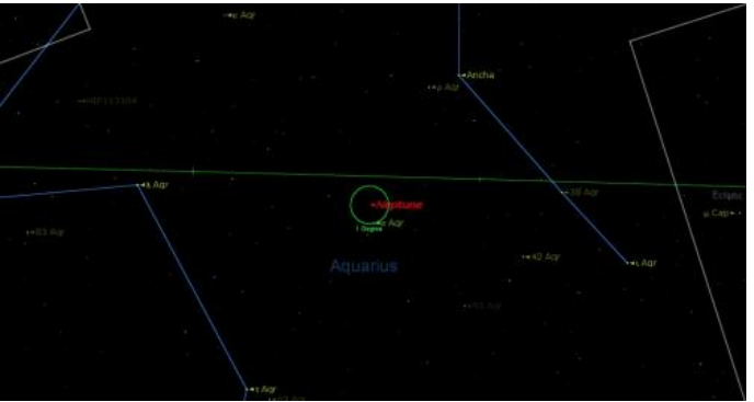
Neptune and a one degree field (green) circle. Note that it passes the bright naked eye star Sigma Aquarii on September 15th. Created using Starry Night Education Software.
