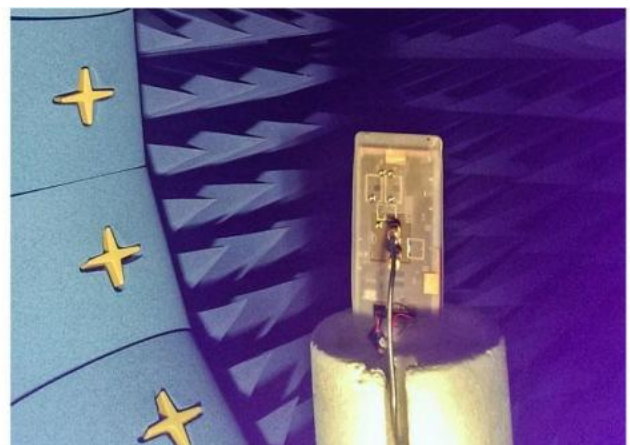
A demonstrator for a handset equipped with frequency reconfigurable antennas.
