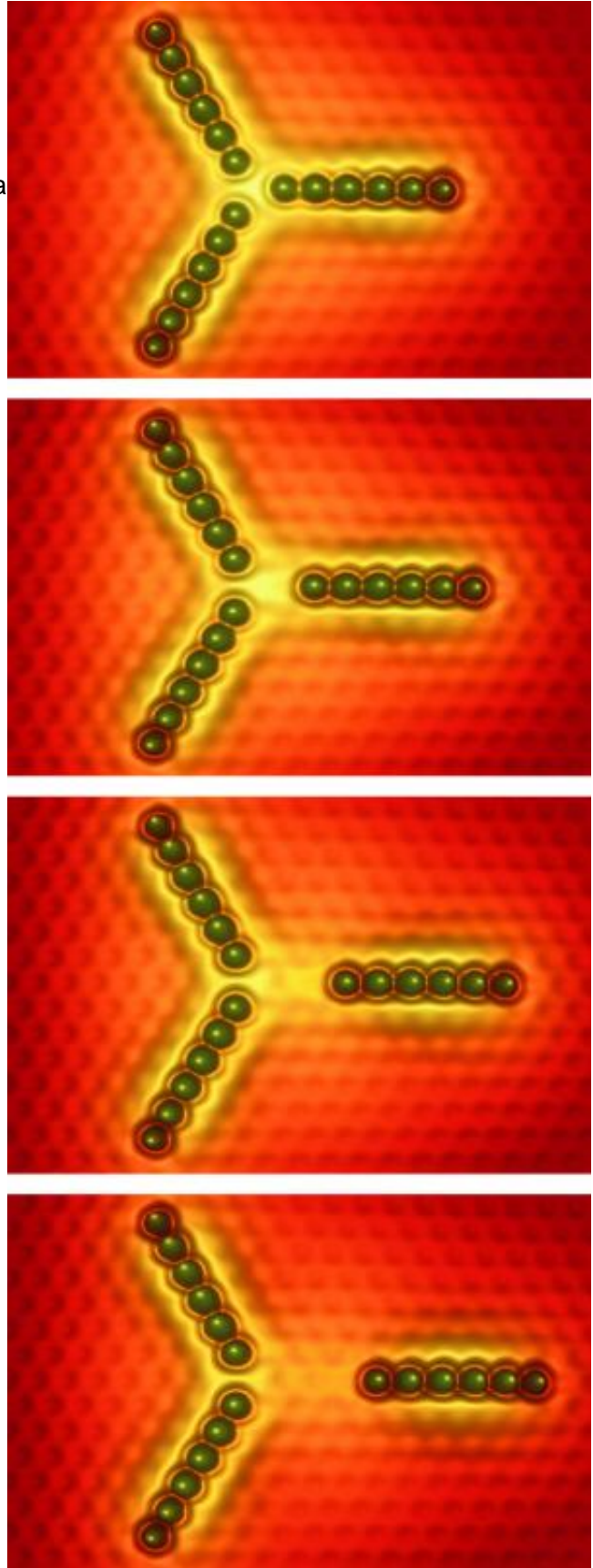
This image shows a quantum dot "molecule" consisting of three 6-atom indium chains. In the top panel, the
