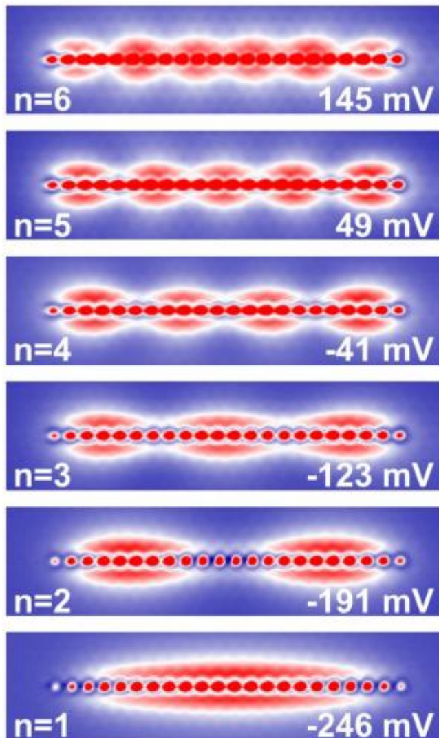
This image shows quantized electron states, for quantum numbers n = 1 to 6 , of a linear quantum dot consisting of 22 indium atoms positioned on the surface of an InAs crystal. Credit: Stefan Fölsch/PDI
