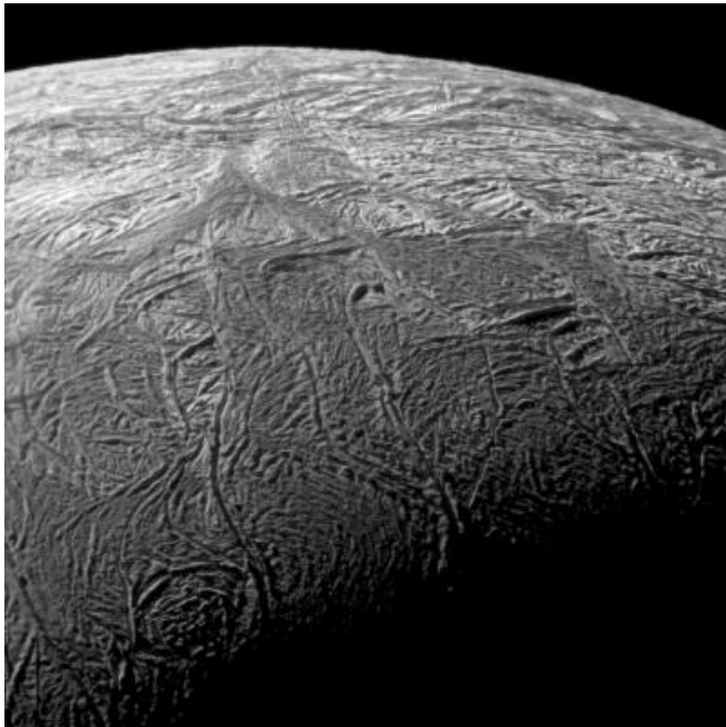
This is a mosaic of images showing cracks in Saturn's moon Enceladus taken by the Cassini spacecraft during its close flyby on March 9 and July 14, 2005. Credit: NASA/JPL/Space Science Institute
