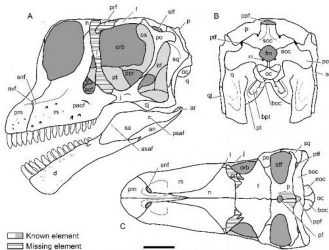
Europasaurus holgeri skull reconstruction in A, left lateral; B, occipital; and C, dorsal views.
