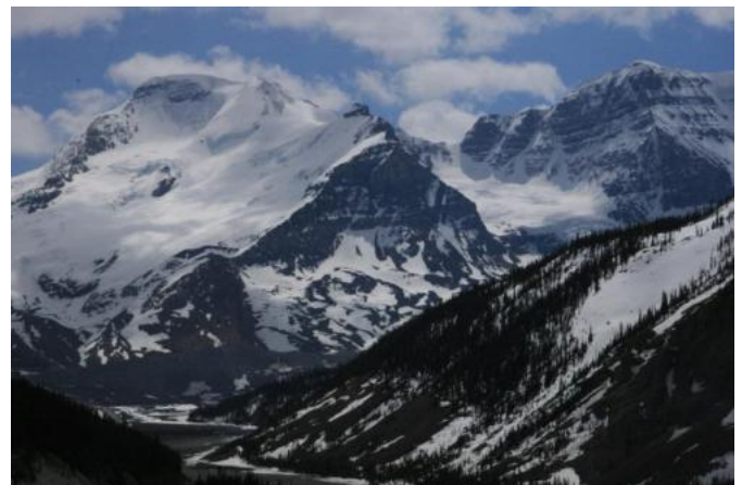
Headwaters of Tsitika River watershed on Northern Vancouver Island, British Columbia, December 2005. Temperature increases will affect the hydrological system in particular in rain/snow transition zones. Credit: Markus Hrachowitz
