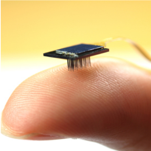
The compact neural probe array consists of a three-dimensional probe array, a custom 100-channel neural recording chip and a flexible polyimide polymer cable. Credit: A*STAR Institute of Microelectronics
