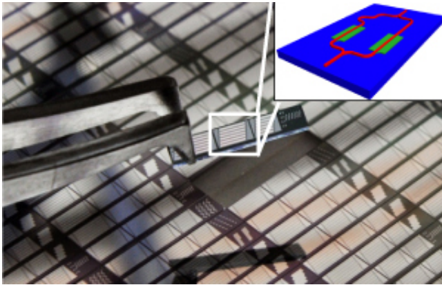
A typical modulator consists of two optical waveguides etched into a silicon chip. Credit: A*STAR Institute of Microelectronics
