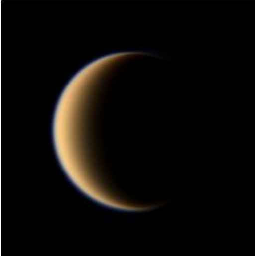
Titan's hazy orange globe hangs before the Cassini spacecraft. Image credit NASA/JPL/Space Science Institute.
