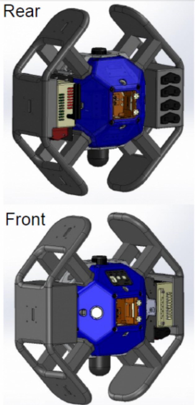
This computer-aided design illustrates the SPHERES-Inspire II Halo interface, which adds processing power and data handling capabilities to SPHERES for testing scenarios aboard the International Space Station. Credit: MIT/Space Systems Laboratory
