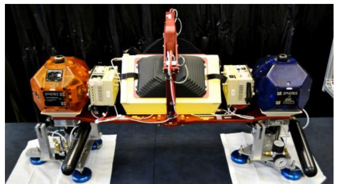
Pill-shaped tanks partially filled with water are attached to the small satellites for the SPHERES-Slosh investigation aboard the International Space Station to simulate the movement of rocket fuels as they slosh inside the tanks.
