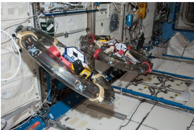
DOD SPHERES-Rings fly freely on the International Space Station during demonstration testing of electromagnetic formation flight and wireless power transfer in microgravity. Credit: NASA
