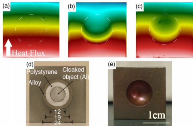
(a) Temperature distribution in a uniform medium connecting a hot (bottom) and a cold region (top). (b) The distribution is distorted in the presence of an obstacle (an air bubble in this example). (c) Adding a thermal cloak restores the transient diffusion and isothermal lines all around the obstacle. (d) Cross section of sample used by Han et al. [1]. (e) Cross section of molded cloak used by Xu et al. [2]. Credit: Physics Viewpoint, DOI: 10.1103/Physics.7.12
