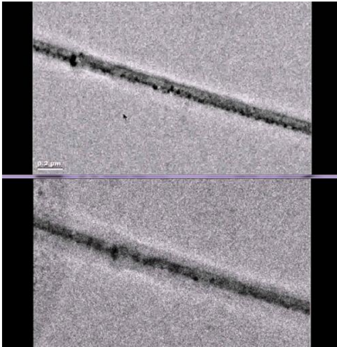
Liquid battery electrolytes makes this view of an uncharged electrode (top) and a charged electrode (bottom) a bit fuzzy. Credit: Gu, et al., Nano Letters 2013
