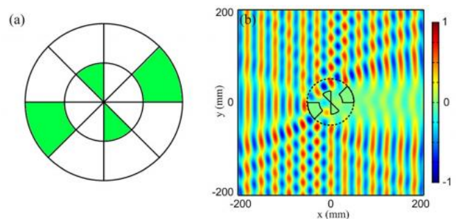
(a) Illustration of a locally invisible object, in which the green subregions are visible and the white subregions are invisible. (b) The near-field distribution of the object enclosed by the localized invisibility cloak shows that the white subregions look like the background, while the green subregions have a solid (visible) appearance. Credit: Jiang, et al. ©2013 AIP Publishing LLC
