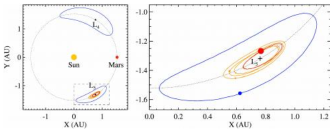
Left (same as Figure 1): The paths traced by all seven Martian Trojans around L4 or L5 (crosses) in a frame rotating with the average angular speed of Mars (red disk) around the Sun (yellow disk). A full revolution around the corresponding Lagrange point takes approximately 1,400 years to complete. The dotted circle indicates the average distance of Mars from the Sun. Right: Detail of left panel (demarcated by the dashed rectangle) showing the motion, over 1,400 years, of the six L5 Trojans: 1998 VF31 (blue), Eureka (red), and the objects identified in the new work (amber). Note the latter's similarity to the path of Eureka. The disks indicate the estimated relative sizes of the asteroids.
