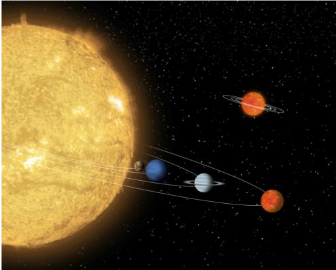
The smallest of several planets in the 55 Cancri system, the former 'diamond planet' is seen orbiting its host star at very close range in this artist's impression. A nearby brown dwarf with its own 'miniature' planetary system is pictured as well. Credit: NASA/JPL-Caltech
