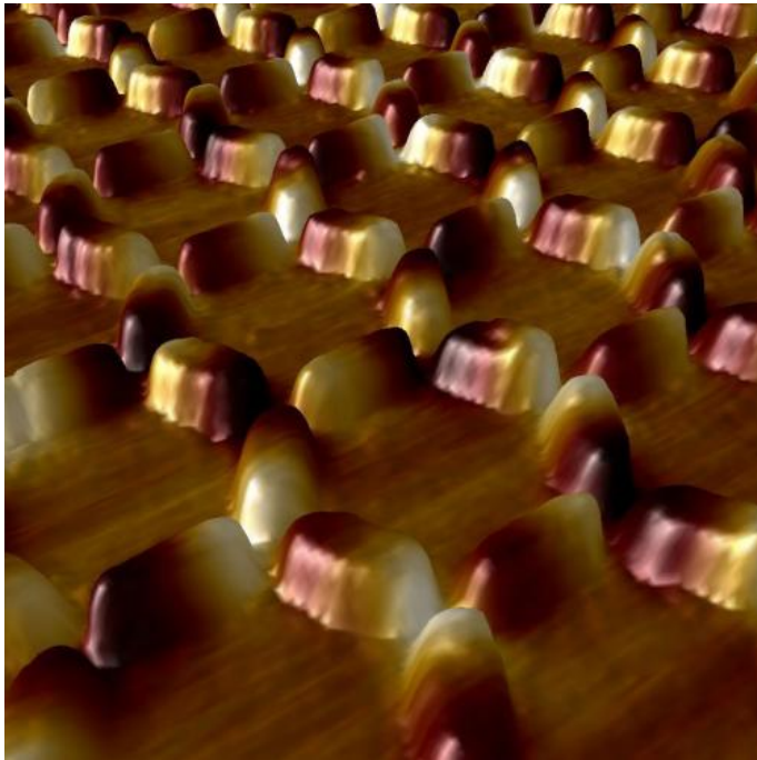
This is a 3-D depiction of the honeycomb artificial spin ice topography after the annealing and cooling protocols. The light and dark colors represent the north and south magnetic poles of the islands. Credit: Ian Gilbert, U. of I. Department of Physics and Frederick Seitz Materials Research Laboratory
