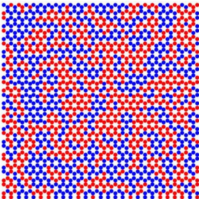
This is a map of the crystallites of ordered magnetic charges in honeycomb artificial spin ice. Red and blue dots correspond to vertices belonging to each of the two degenerate magnetic charge-ordered states. Credit: Ian Gilbert, U. of I. Department of Physics and Frederick Seitz Materials Research Laboratory
