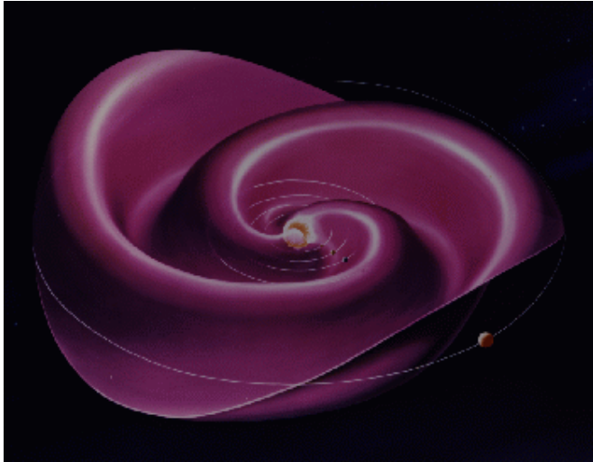
An artist's concept of the heliospheric current sheet, which becomes more wavy when the sun's magnetic field flips.
