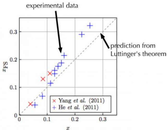
Graph showing the breakdown of Luttinger's theorem in the normal state of cuprate superconductors. The horizontal axis is the expected number of mobile electrons while the vertical axis is the measured number. The two should be equal if the theorem were true. Credit: Philip Phillips
