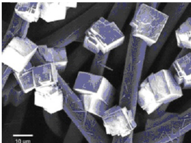
Scanning electron microscopy image of cubic Na 2 O 2 particles on the cathode after cell discharge. Image credit: P. Hartmann
