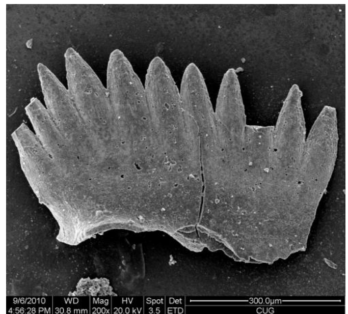
Scanning electron microscope image that shows an Early Triassic conodont, a fossil from an eel-like marine animal, that is used for oxygen isotope measurement and past temperature reconstruction. Credit: Yadong Sun
