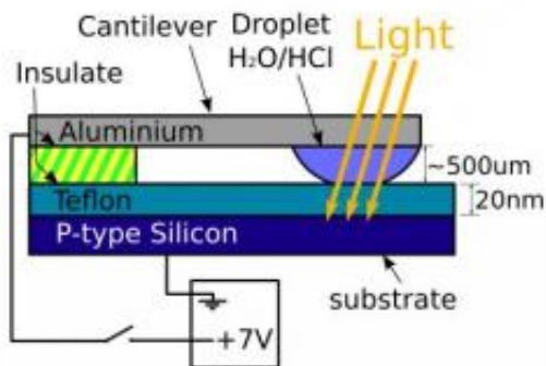
Experimental setup showing aluminum cantilever, liquid droplet (H 2 O/HCl, c = 0.01\text{M} ) and Teflon AF/silicon photoelectrowetting surface. Image from arXiv:1201.2873v1.
