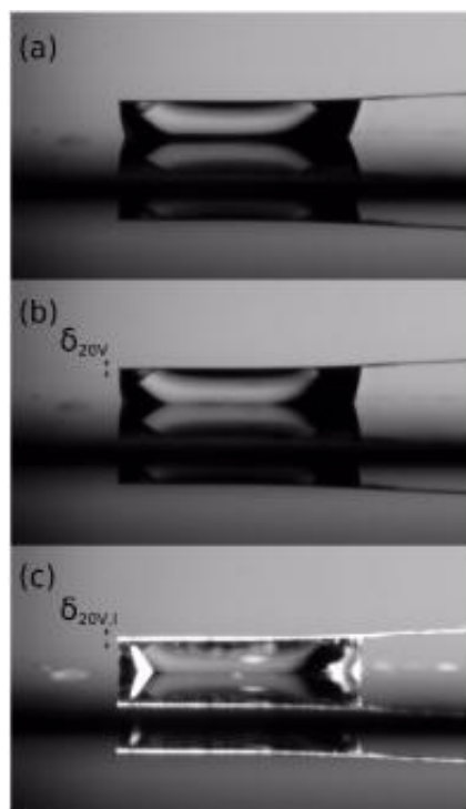
Deflection of a 30\mu\text{m} thick Al cantilever using photoelectrowetting on a Teflon AF (265 nm)/p-type silicon ( NA = 1.8 \times 10^{15} \text{ cm}^{-3} ) stack at (a) 0V (dark), (b) +20V (dark) and (c) +20V (illuminated). Image from arXiv:1201.2873v1
