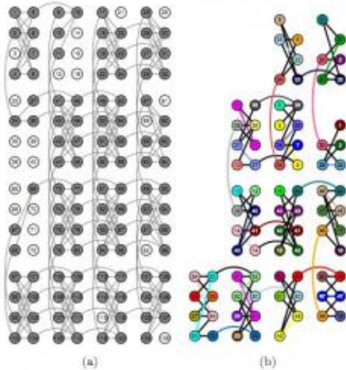
(a) Layout of qubits and couplers. (b) R(8, 2) embedding for qubit connectivity. Image: arXiv:1201.1842v2 [quant-ph]
