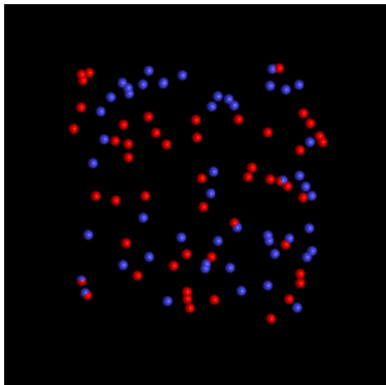
Electrons (blue balls) and holes (red balls) show random thermal motion before the terahertz pulse hits the sample. Copyright: MBI
