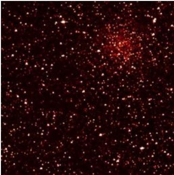
An image taken by Kepler of star cluster NGC 6791, which is located 13,000 light years from Earth. The image has been color-coded so that brighter stars appear white, and fainter stars, red. Image credit: NASA/Ames/JPL-Caltech
