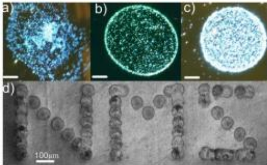
Dark field optical micrograph of inkjet printed drops on a) plasma cleaned, b) pristine and c) HMDS treated substrate. Scale: 20 \mu m. d) SEM micrograph of printed pattern. Image from arXiv:1111.4970v1 [cond-mat.mtrl-sci]
