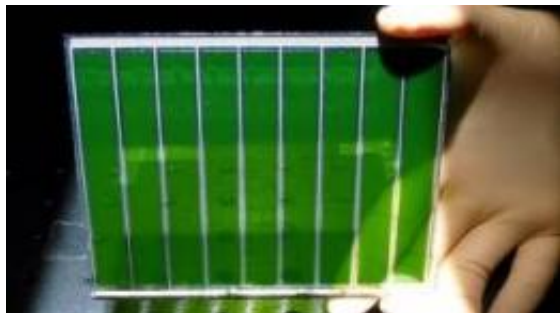
Green dye-sensitized solar cells © 2011 EPFL
