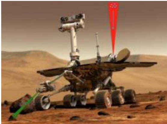
Goddard technologists are studying different techniques for corralling particles and transporting them via laser light to instruments on rovers and orbiting spacecraft. Credit: Concept image courtesy Dr. Paul Stysley
