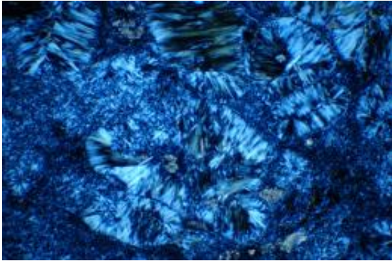
A photomicrograph of a thin section of serpentine rock. Photos by Emily Pope
