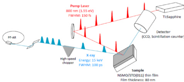
Fig. 1: Experimental setup of 100-ps TR-XRD.
