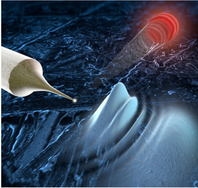
A tungsten tip is irradiated with a laser pulse (indicated by a red ball). The blue wave illustrates the interference pattern of the two electrons emitted from the tip. Credit: Christian Hackenberger
