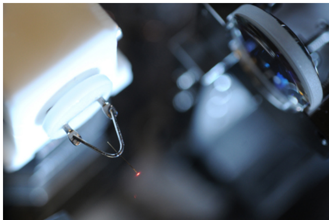
Metal tip irradiated with a laser pulse. Credit: Thorsten Naeser, MPQ
