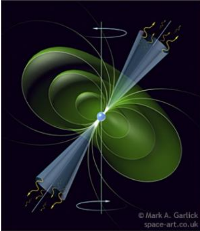
Pulsar diagram Credit: Mark Gartlick
