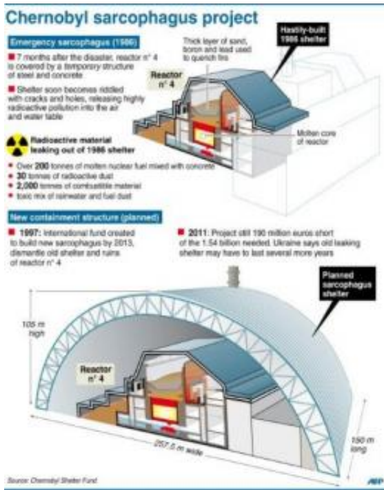
Graphic illustration of the ageing containment structure covering the destroyed reactor at Chernobyl and plans to build a new sarcophagus over it
