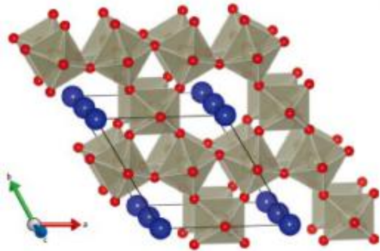
Figure 1: The crystal structure of Hg_xReO_3 . The mercury (Hg) atoms are shown in blue, oxygen (O) in red and rhenium (Re) in brown. Credit: 2011 The American Physical Society
