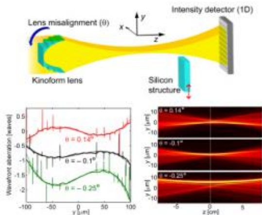
Top: Experimental setup. Bottom: Measured and simulated lens aberrations (left) and their corresponding through focus amplitude of reconstructions (right) for different lens angular misalignments. (From Manuel Guizar-Sicairos et al., Appl. Phys. Lett. 98, 111108 [2011]. © 2011 American Institute of Physics)
