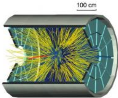
This 3D illustration of the STAR Time Projection Chamber shows the track of an antihelium-4 nucleus (red). Image credit: STAR Collaboration, RHIC, Brookhaven National Laboratory.
