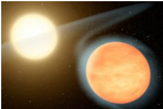
Artist concept of the extremely hot exoplanet WASP-12b and the host star. Image: NASA/JPL-Caltech/R. Hurt (SSC)
