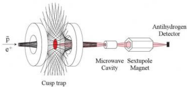
Conceptual experimental setup for ground-state hyperfine transition measurements of antihydrogen atoms with the cusp trap.
