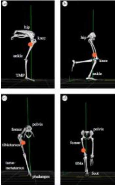
Human and ostrich hind-limb postures during mid-stance of running: (a,b) sagittal plane; (c,d) frontal plane. Image: [i]Journal of the Royal Society Interface[/i], doi:10.1098/rsif.2010.0466
