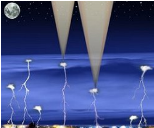
An artist's concept of TGFs. Credit: NASA/Robert Kilgore
