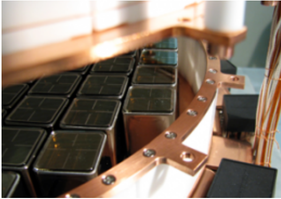
Some of the light sensors that make up the lower detector on the XENON experiment. Image credit: Guillaume Plante
