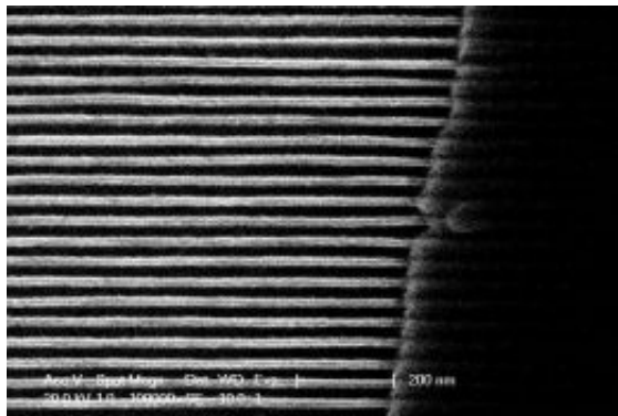
An array of YBCO nanowires with 20-nanometer diameters. Image courtesy of James Heath.
