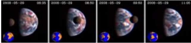
Series of images showing the Moon transiting Earth, captured by NASA's EPOXI spacecraft. Credit: Donald J. Lindler, Sigma Space Corporation/GSFC; EPOCH/DIXI Science Teams
