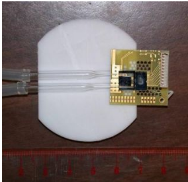
Prototype microchip device combining NIST's miniature atomic magnetometer with a fluid channel for studies of tiny samples. Credit: NIST
