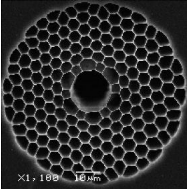
Electron microscope image of the hollow-core fiber. Credit: University of Bath
