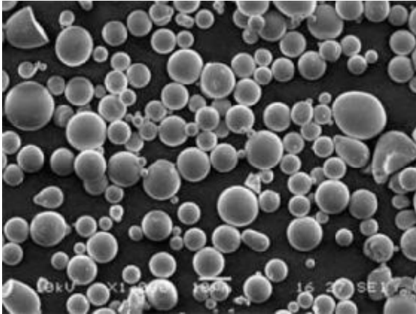
An micrograph of the fine, spherical 2-14-1 permanent magnet alloy powders produced by argon gas atomization. Credit: US DOE's Ames Laboratory
