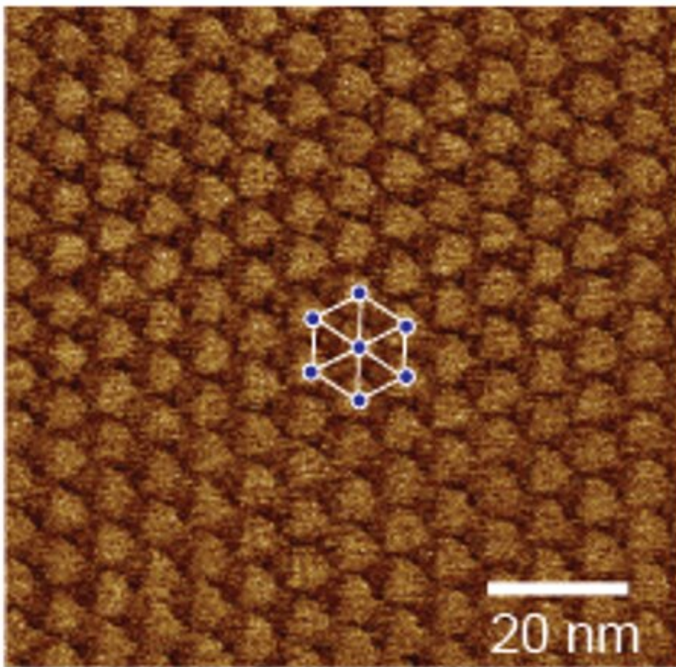
A top-view image, taken by piezoresponse force microscopy, of stacked layers of tungsten diselenide and tungsten disulfide, forming what is known as a heterostructure. Triangles indicate the repeating "units" of the moiré superlattice. Credit: Xi Wang/University of Washington
