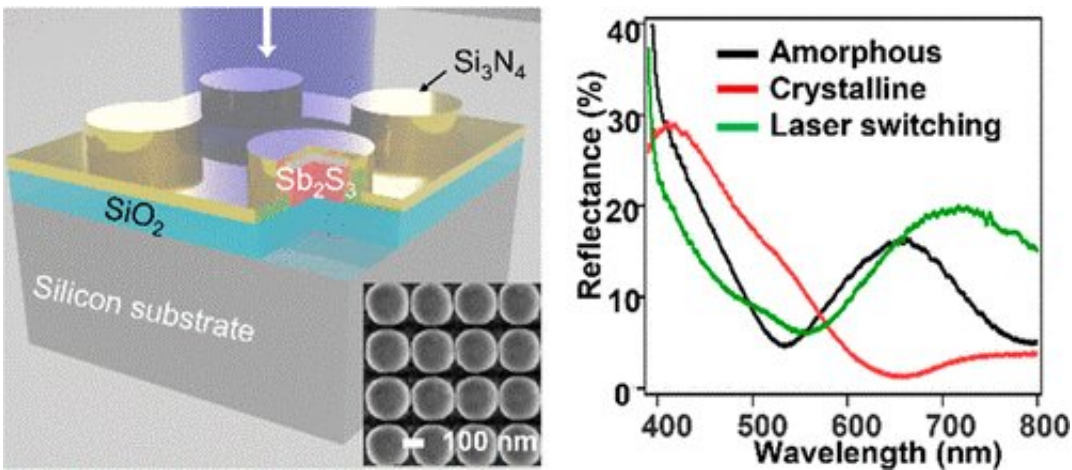
Illustration of the antimony trisulphide programmable metasurface and its reflection spectrum in multiple states. Credit: SUTD
